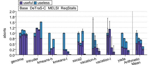
Fig. 12: Distribution of conflict-induced aborts.
