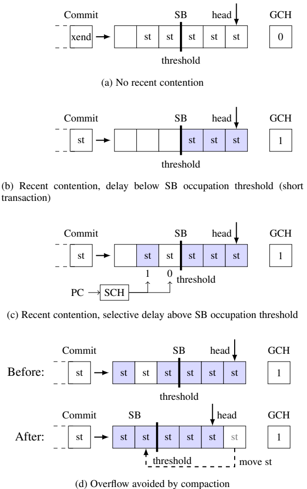
Fig. 3: Overflow avoided with compaction.
