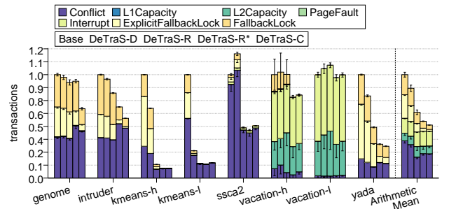
Fig. 8: Aborted transactions by cause.
