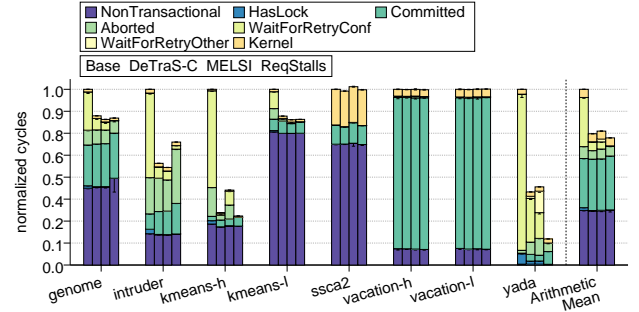
Fig. 11: Normalized execution time breakdown.
