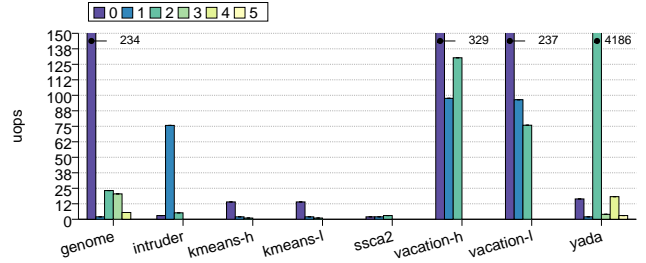
Fig. 7: Store micro-ops in STAMP, per transaction xid .
