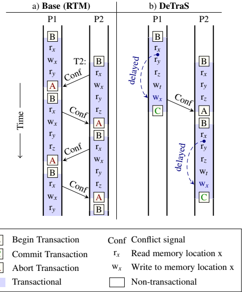
Fig. 2: Motivation for delaying transactional stores. Left: typical friendly-fire scenario in requester-wins HTM designs. The transaction comprises the following accesses: r_x , w_x , r_y , r_z , w_t . Right: friendly-fire mitigation by delaying w_x .
