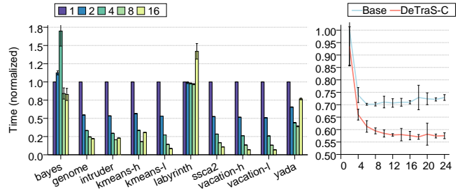
Fig. 4: Left: Execution time in Base up to 16 threads, normalized to sequential. Right: Sensitivity analysis for maximum number of retries before acquiring fallback lock.
