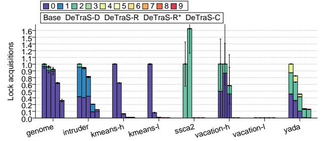
Fig. 6: Acquisitions of the fallback lock, per xid .
