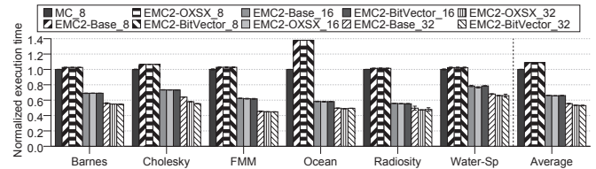
Fig. 13. Normalized execution time.
