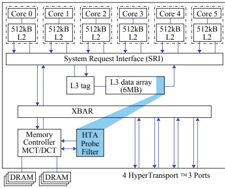
Fig. 1. Block diagram of Magny-Cours dies [4].
