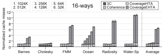
Fig. 17. Normalized number of cache misses when the EHTA size is reduced from 1024K entries to 32K entries.
