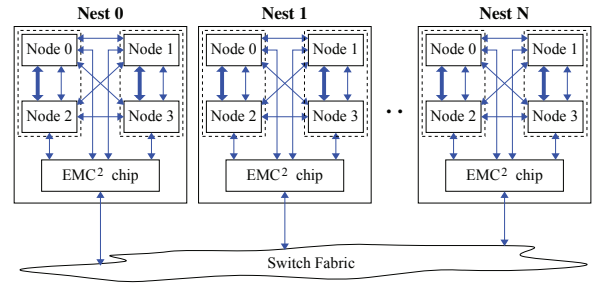
Fig. 2. Overview of the proposed system. Thick arrows inside the nests represent x16 cHT links while the narrow ones are x8 cHT links.
