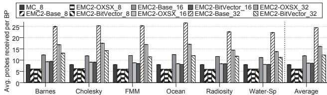
Fig. 11. Number of probes received for each broadcast sent by the home die.
