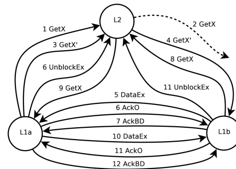
Fig. 6. Transaction where the lost data timeout detects data which have been wrongly discarded. L1a makes a request (1) to L2 which forwards it to L1b. The forwarded message (2) gets delayed in the network, and hence, the lost request timeout triggers in L1a. When this happens, L1a reissues the request (3) which is forwarded again by L2 (4). This time, the request arrives to L1b which sends the data (5) to L1a. When L1a receives the data, it sends (6) an unblock message to L2 and an ownership acknowledgment to L1b which responds with a backup deletion acknowledgment (7) to L1a. Later, L1b makes a new request which is handled in a similar way (messages 8-12), so it has the only copy of the data again with exclusive access. If the first forwarded request (2) arrives now to L1b, it will send the data to L1a which will discard it (since it does not expect a response with that serial number anymore). In this situation, no node will have the data nor expect it; so, future accesses to the line would cause a deadlock.
