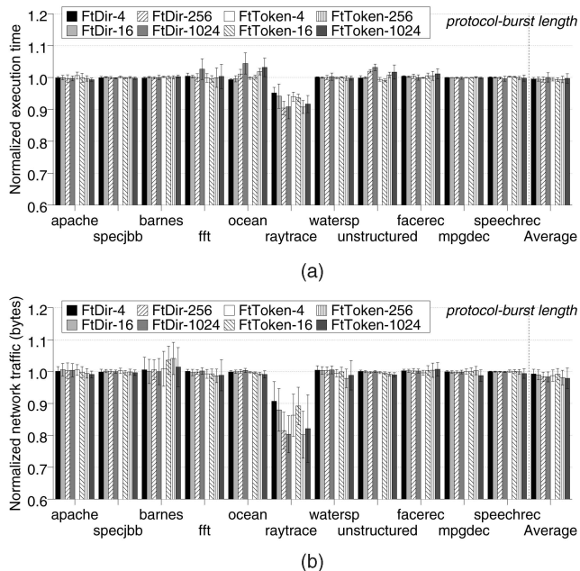
Fig. 8. Relative execution time with burst faults of several lengths with respect to single message faults. The fault rate is fixed to 125 corrupted messages per million. (a) Execution time overhead. (b) Network traffic overhead.
