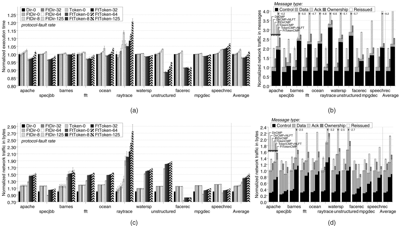
Fig. 7. Execution time and network overhead of each cache coherence protocol compared to DIRCMP. (a) Execution time overhead with several fault rates. (b) Number of messages (no faults). (c) Network overhead (bytes) with several fault rates. (d) Bytes transmitted (no faults).
