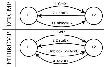
Fig. 3. Message exchange for an L1 write miss that hits in L2. In both protocols, the L1 cache sends a GetX message (1) to the L2, which has the data in an exclusive state (M or E). In DIRCMP, when L2 receives the request, it sends the data to L1 (2) which, on receipt, transitions to modifiable (M) state and answers to L2 with an UnblockEx message. In FTDIRCMP, when L2 receives the request, it sends the data to L1 (2) but it also keeps a backup copy of the data. When L1 receives the data, it transitions to blocked ownership and modifiable (Mb) state and answers with a message (3) which serves both as the UnblockEx and as the AckO messages used in Fig. 2. The backup copy in L2 will be kept until the UnblockEx+AckO message sent by L1 is received and the AckBD message (4) is sent to L1, which transitions to the modifiable (M) state on receipt.
