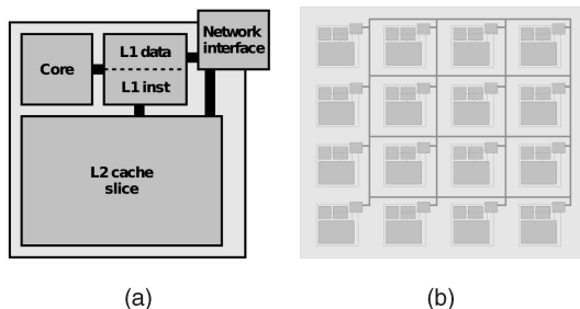
Fig. 1. Tiled chip multiprocessors. (a) Diagram of an individual tile. (b) 16-Way tiled CMP with 2D mesh interconnection network.
