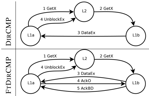
Fig. 2. Message exchange for a cache-to-cache write miss. Initially, for both protocols, L1b has the data in modifiable (M), exclusive (E), or owned (O) state and L1a requests write access to L2 (1) which forwards the request to L1b (2). In DIRCMP, L1b sends the data to L1a (3) and transitions to invalid state. Subsequently, when L1a receives the data, it transitions to a modifiable (M) state and sends an UnblockEx message to L2. In FTDIRCMP, when L1b receives the forwarded GetX , it sends the data to L1a and transitions to the backup state (3). When L1a receives the data, it transitions to the blocked ownership and modifiable (Mb) state and sends the UnblockEx message to L2 and an AckO message to L1b (4). When L1b receives the AckO , it discards the backup data, transitions to invalid (I) state, and sends an AckBD message to L1a (5), which transitions to the usual modifiable (M) state on receipt.
