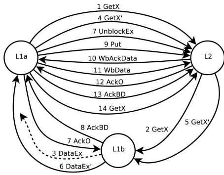
Fig. 5. Transaction where request serial numbers avoid using stale data. L1a makes a request (1) to L2 which forwards it to L1b (2). L1b sends the data (3) to L1a, but this message gets delayed in the network for such a long time that the request timeout triggers and L1a reissues the request (4) which is forwarded again to L1b (5) which has a backup copy of the data and resends it (6). This time, it arrives at L1a which sends (7) an unblock to L2 and an ownership acknowledgment to L1b. L1b answers with a (8) backup deletion acknowledgment to L1a. After modifying the data, L1a performs a writeback to L2 (messages 9-13), and after that, it issues another request (14). If the first data message (3) arrives at this moment and is not discarded using its serial number, it would allow L1a to use the old data.
