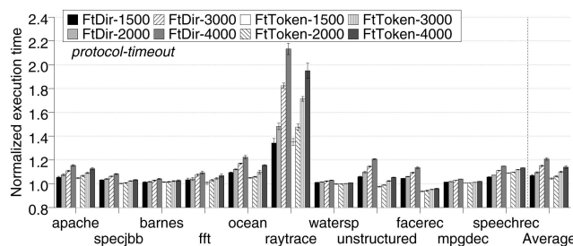
Fig. 9. Relative execution time with respect to DIRCMP without faults for each fault-tolerant protocol with 250 corrupted messages per million using different values for the fault detection timeouts.
