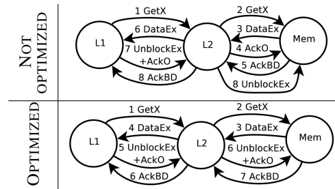
Fig. 4. L2 miss optimization of ownership transference. In both cases, the L1 sends a GetX message (1) to L2 which, since it does not have the data, forwards (2) it to the memory controller. The memory controller fetches the data and sends it to L2 using a DataEx message (3). Now, in the unoptimized case, when the L2 receives the owned data, it sends an ownership acknowledgment (4) to the memory controller and waits for the backup deletion acknowledgment (5) before answering to L1 with the data (6). Once L1 receives the data, it sends a message to L2 (7) carrying the ownership acknowledgment and the unblock. When L2 receives this message, it will send a backup deletion acknowledgment to L1 and an unblock message to the memory controller (8). On the other hand, in the optimized version, when L2 receives the DataEx (3) message from memory, it sends another DataEx (4) to L1. Notice that now the critical path of the miss requires only 4 hops instead of 6. Once the L1 has received the data, it will send a message (5) with the unblock and the ownership acknowledgment to L2 which will then send the unblock to memory and the backup deletion acknowledgment to L1 (6). Finally, when the memory controller receives the ownership acknowledgment, it will answer with a backup deletion acknowledgment message (7).
